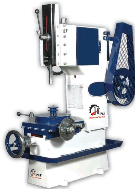
6" STROKE LIGHT DUTY MODEL
